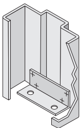
ONE PIECE WELDED BASED ANCHOR
