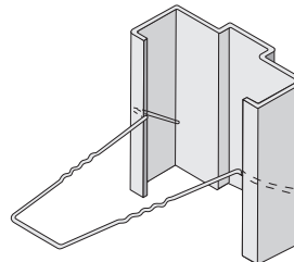
MASONRY WIRE ANCHOR
