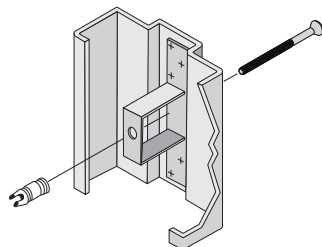
EXISTING OPENING ANCHOR (E.O.A.)
