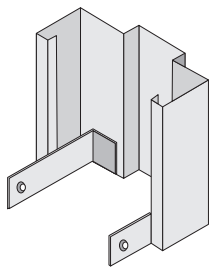
STRAP ANCHOR
